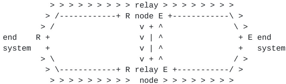
Figure 1: Packet replication and elimination
