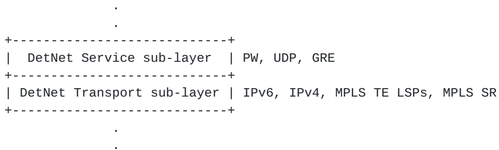
Figure 4: DetNet adaptation to data plane
