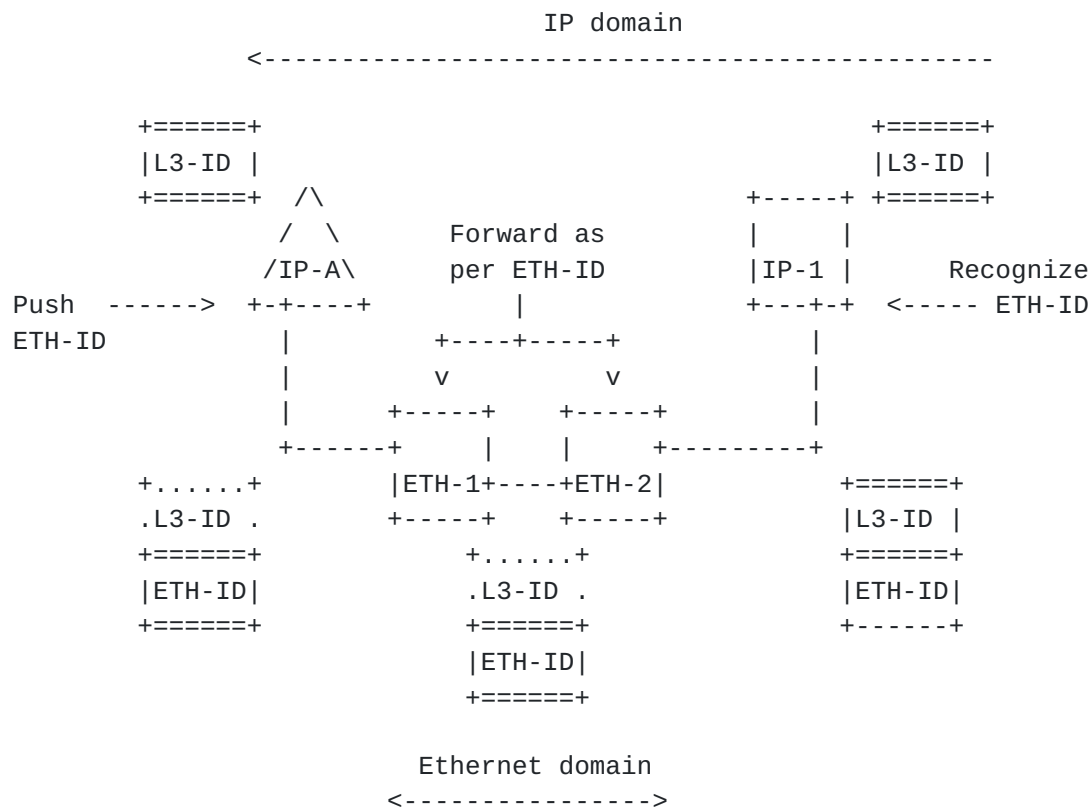
Figure 10: IP nodes interconnected by an Ethernet domain
