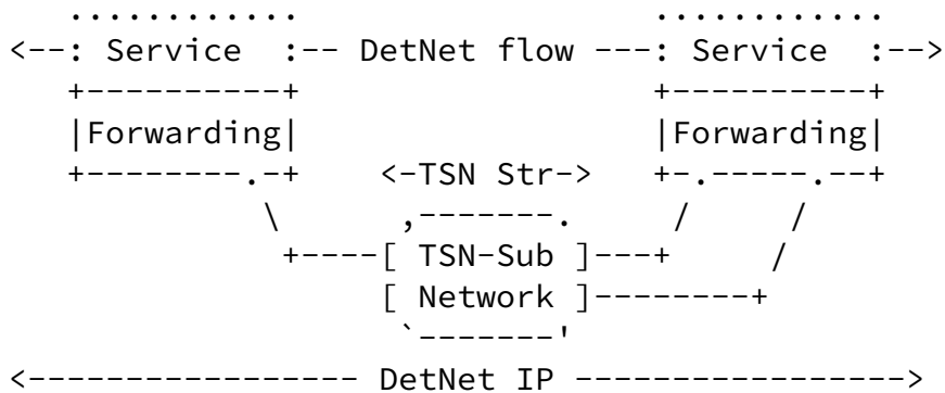
Figure 1: DetNet (DN) Enabled IP Network over a TSN sub-network
