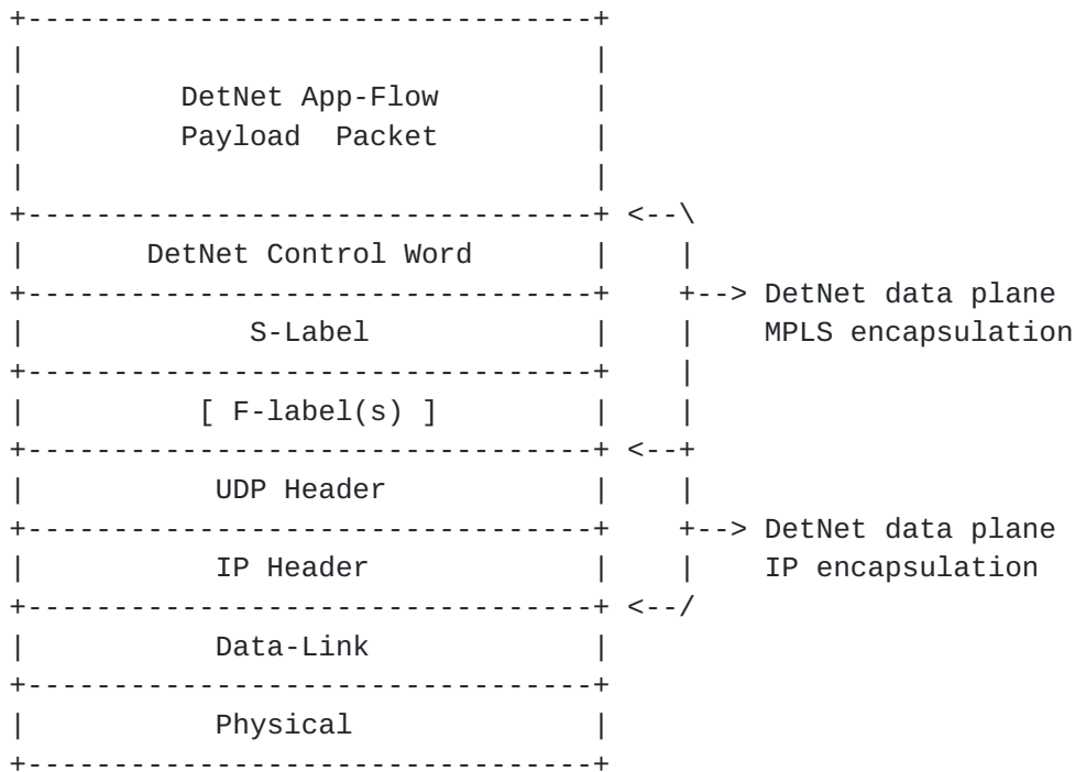
Figure 1: UDP/IP Encapsulation of DetNet MPLS
