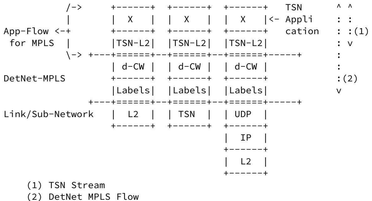
Figure 3: Example TSN over MPLS Encapsulation Formats
