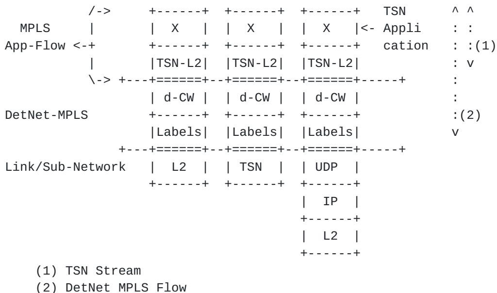
Figure 3: Examples of TSN over MPLS Encapsulation Formats
