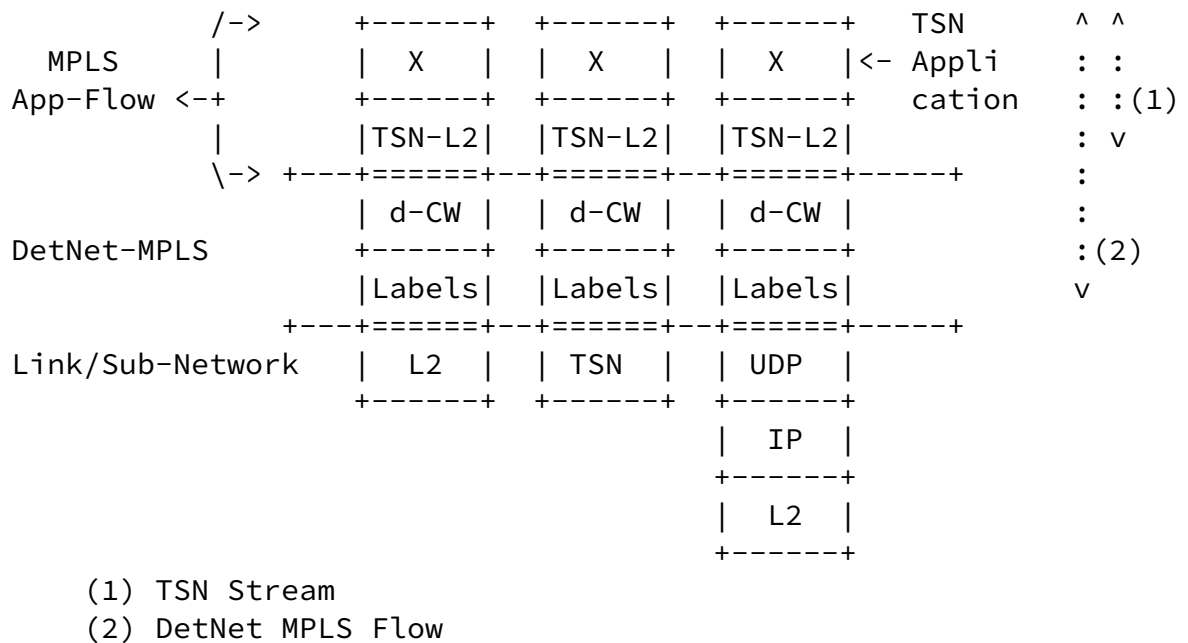
Figure 3: Examples of TSN over MPLS Encapsulation Formats
