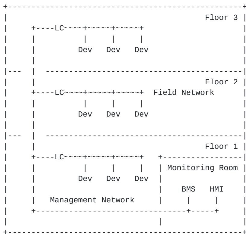
Figure 2: Deployment model for Medium/Large Buildings
