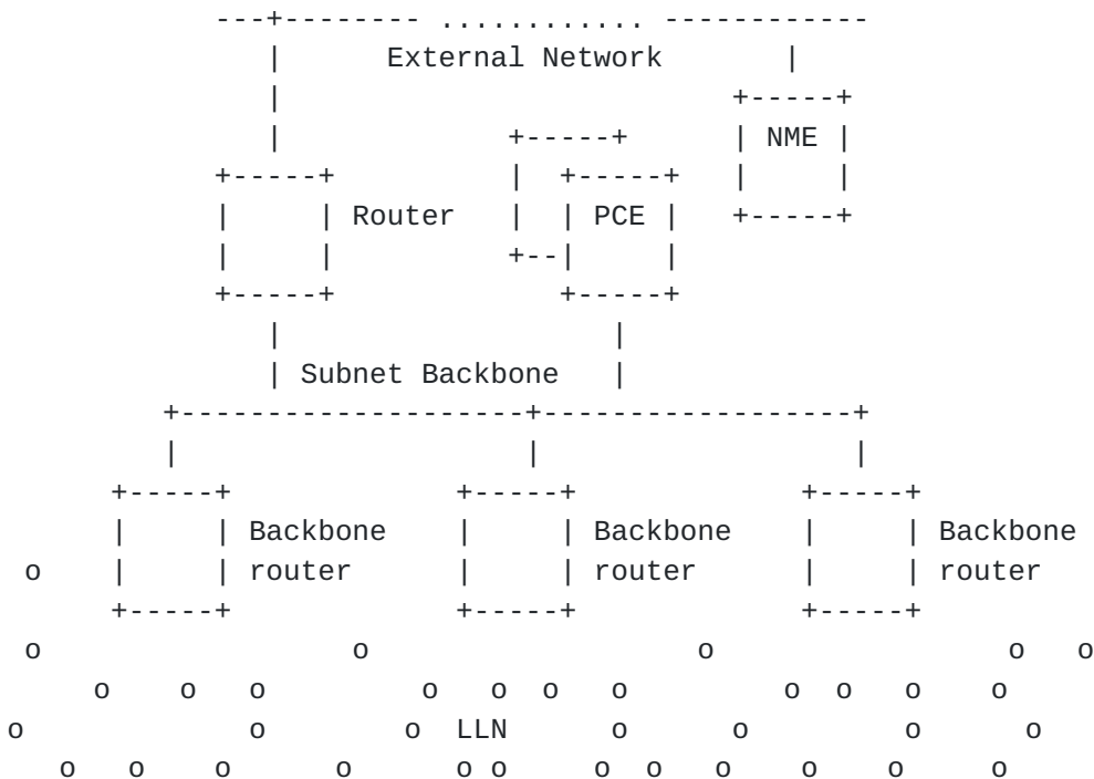
Figure 5: Extended 6TiSCH Network
