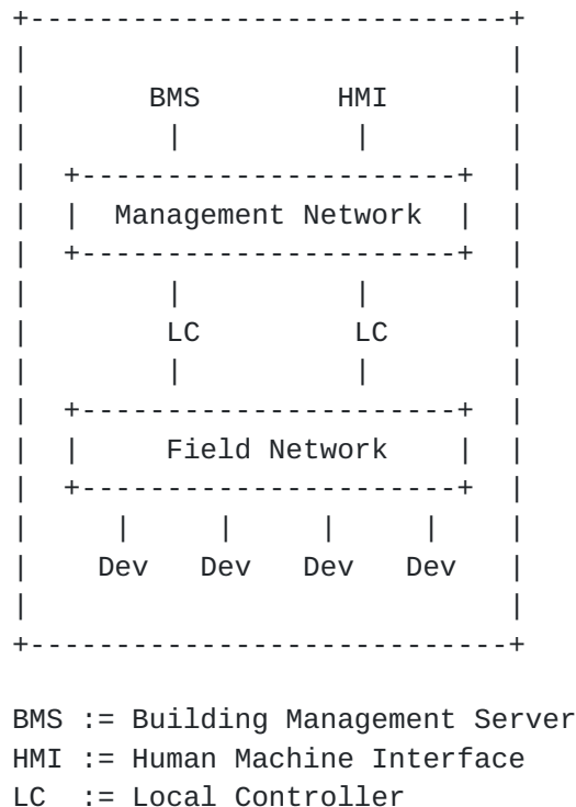
Figure 4: BAS architecture
