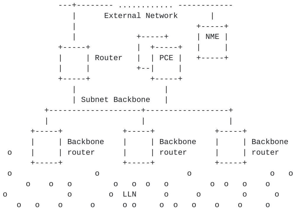
Figure 8: Extended 6TiSCH Network
