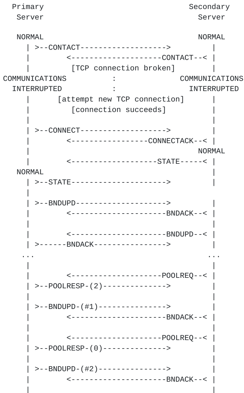
Figure 6: Transition from NORMAL to COMMUNICATIONS-INTERRUPTED and back (example with 2 addresses allocated to secondary)
