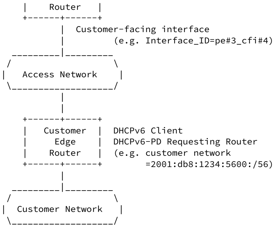
Figure 2: Use case of ISP-Customer network where CPE is connected to PE through access network
