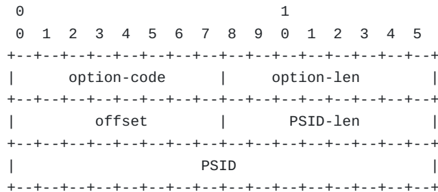
Figure 1: DHCPv4 Port Parameters Option
