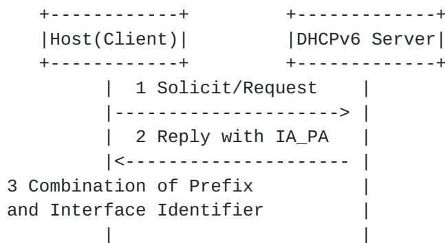
Figure 1: DHCPv6 Operation
