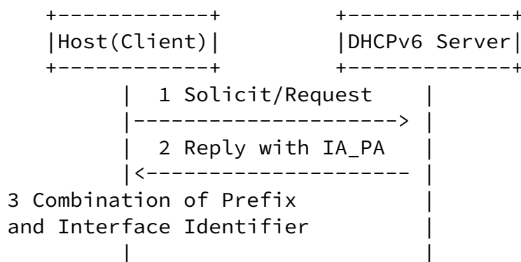
Figure 1: DHCPv6 Operation
