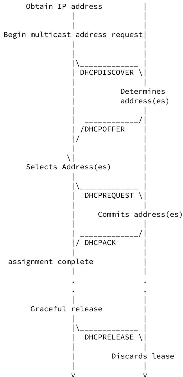
Figure 1: Timeline diagram of messages exchanged between MDHCP client and servers when allocating multicast address(es) using unicast messages to a MDHCP capable server.
