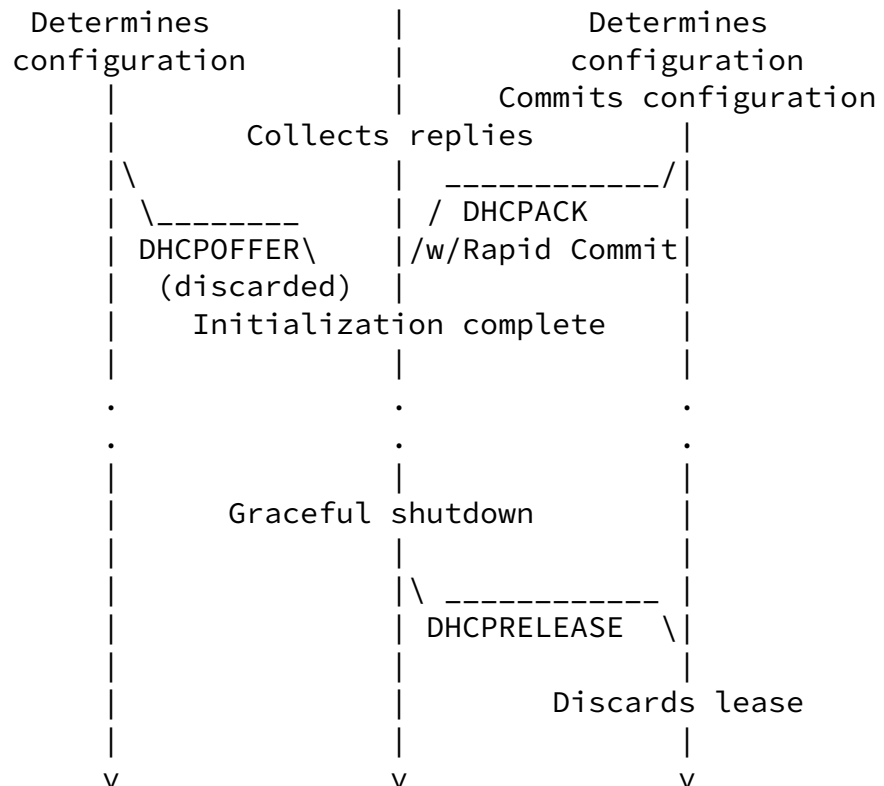
Figure 1: Timeline diagram when Rapid Commit used
