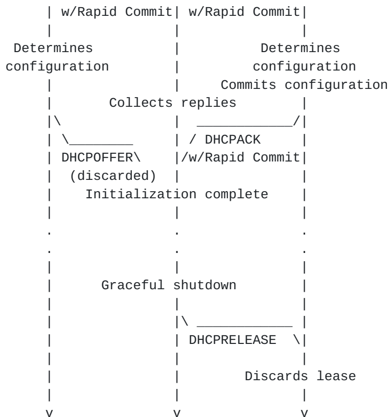
Figure 1: Timeline diagram when Rapid Commit used
