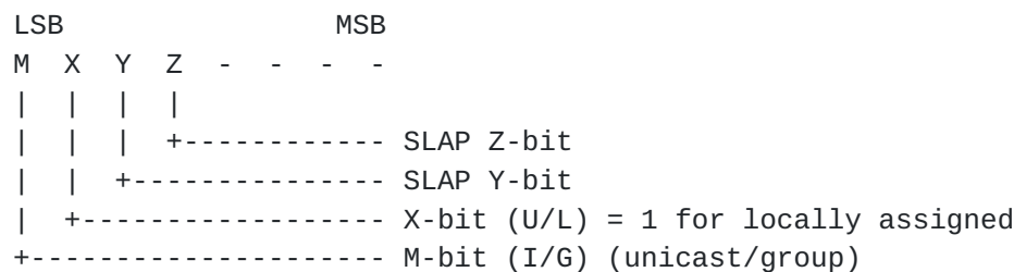
Figure 1: IEEE 48-bit MAC address structure (in IEEE representation)
