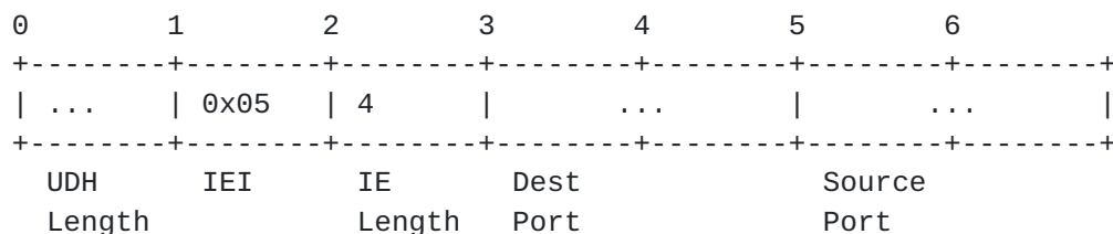
Figure 14: Application Port Addressing Scheme (16 bit address).
