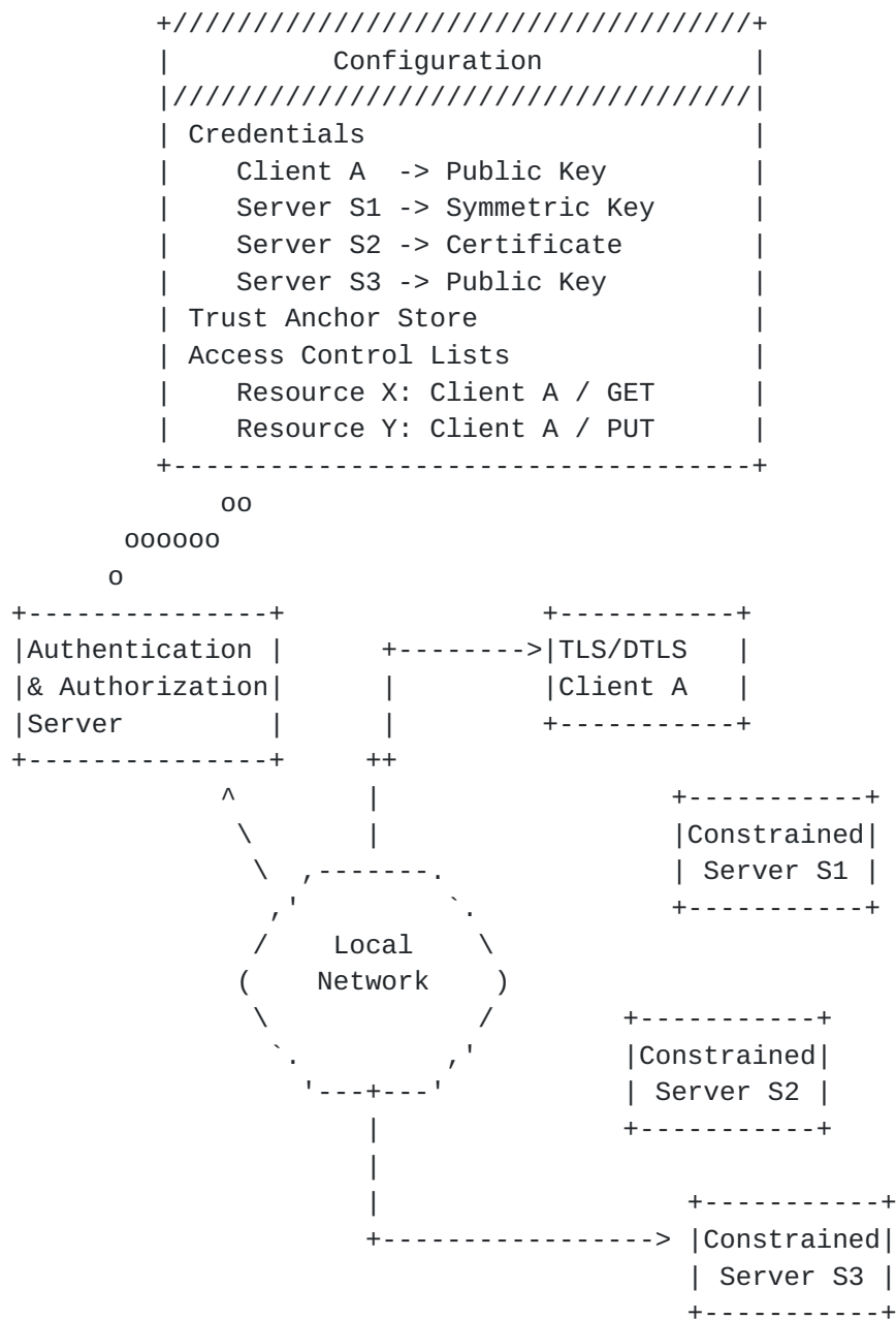
Figure 6: Constrained Server Profile.
