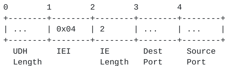
Figure 13: Application Port Addressing Scheme (8 bit address).
