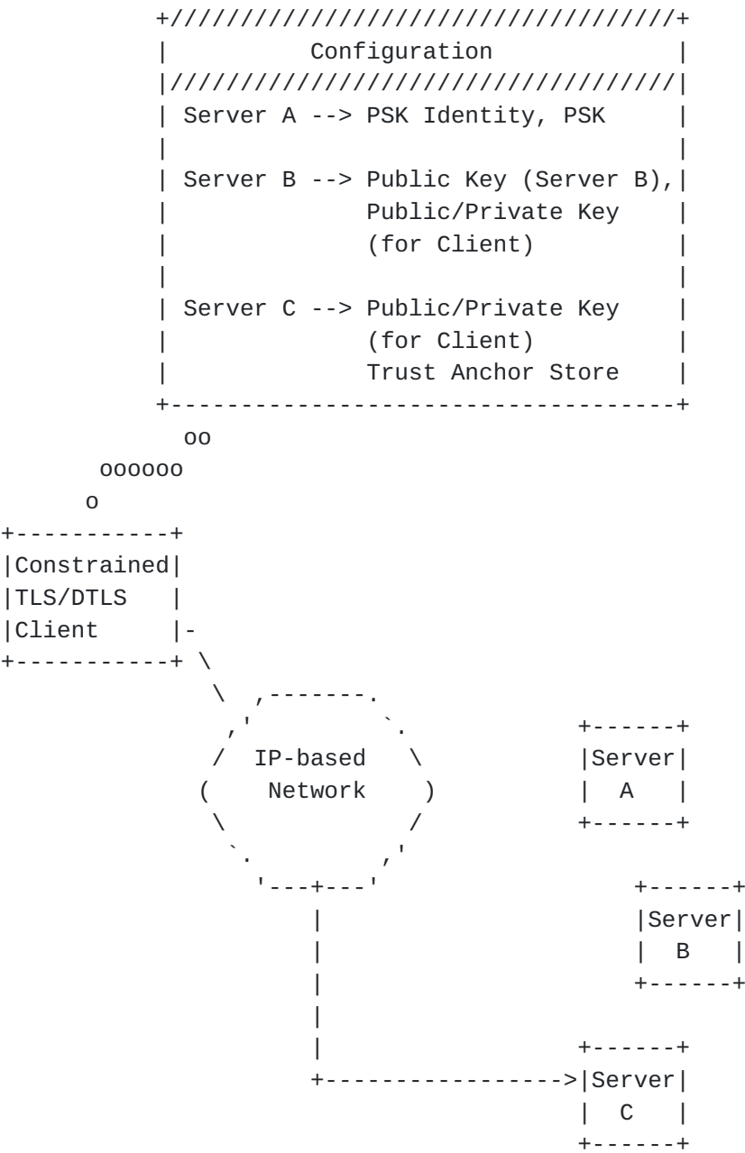
Figure 1: Constrained Client Profile.
