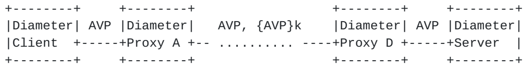
Figure 5: Middle-to-Middle Diameter AVP Security Protection.
