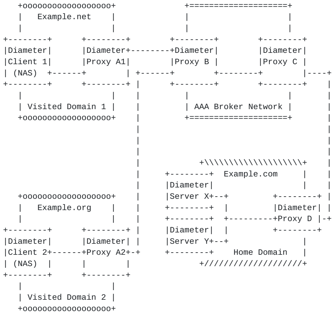
Figure 1: Example Diameter Deployment.
