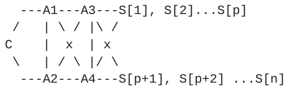
Figure 13: Full Mesh
