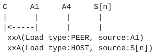
Figure 5: Answer Message from A1
