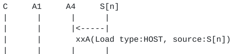
Figure 3: Answer Message from S[n]
