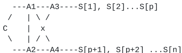
Figure 1: Example Diameter Network
