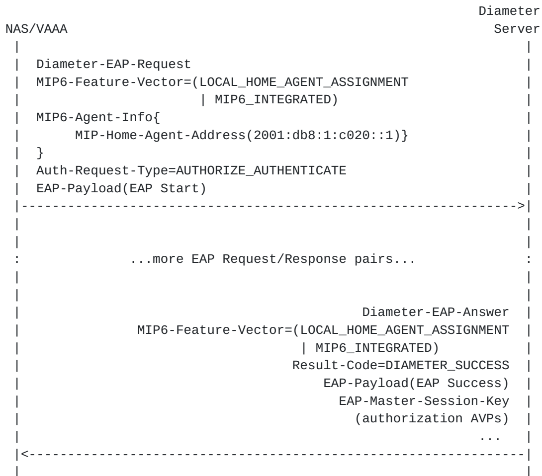
Figure 2: Home Agent Assignment by NAS
