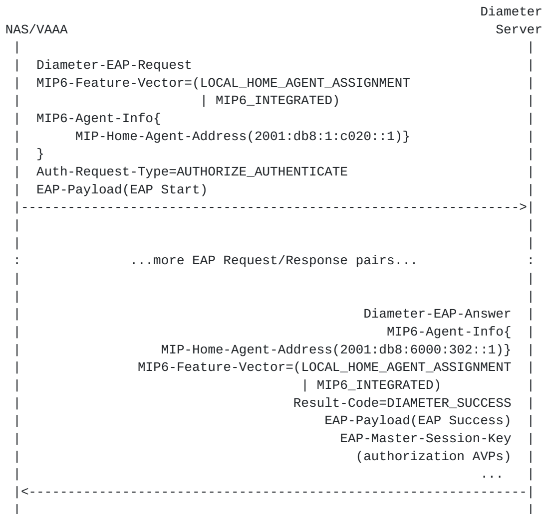
Figure 4: Home Agent Assignment by NAS or Diameter Server
