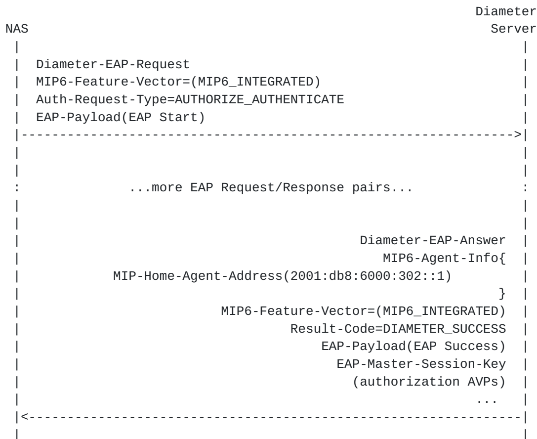
Figure 3: Home Agent Assignment by Diameter Server
