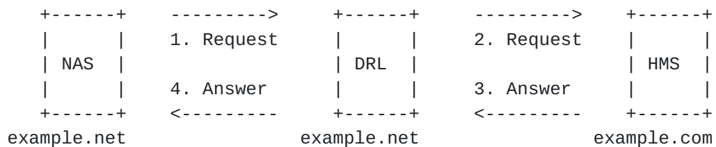
Figure 2: Relaying of Diameter messages
