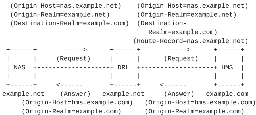
Figure 6: Routing of Diameter messages
