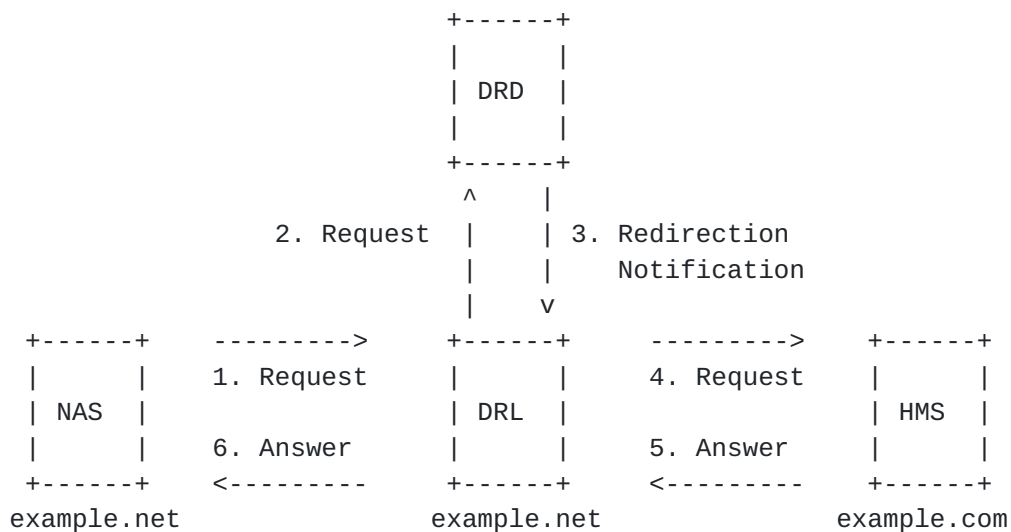
Figure 3: Redirecting a Diameter Message
