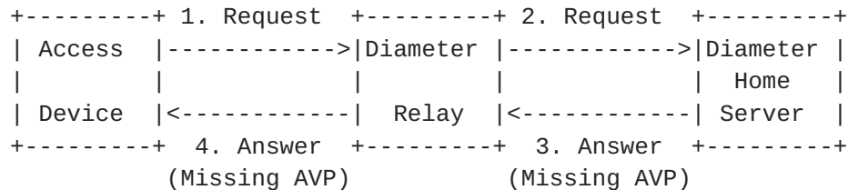
Figure 8: Example of Application Error Answer message
