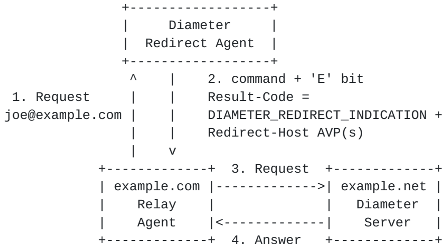
Figure 5: Diameter Redirect Agent
