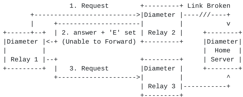
Figure 7: Example of Protocol Error causing answer message
