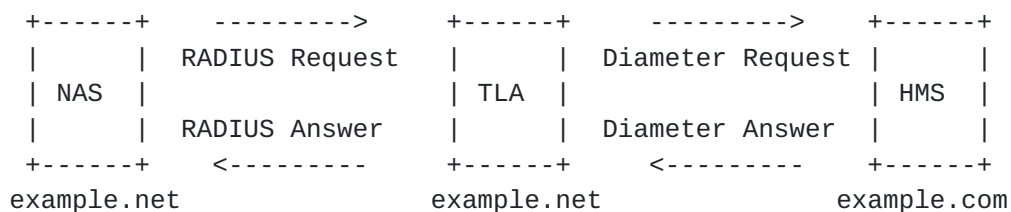
Figure 4: Translation of RADIUS to Diameter
