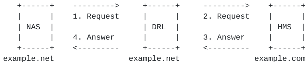
Figure 2: Relaying of Diameter messages
