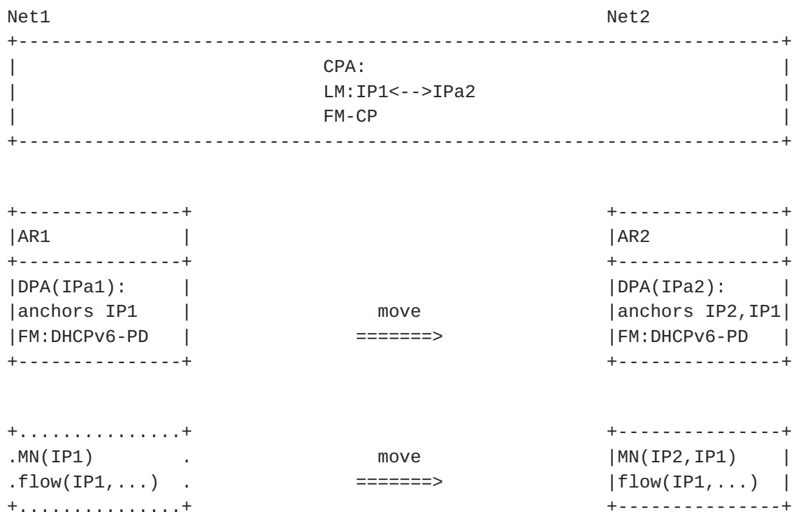
Figure 7. IP prefix/address anchor switching to the new network with LM and FM-CP in a centralized control plane whereas the FM-DP's are distributed.
