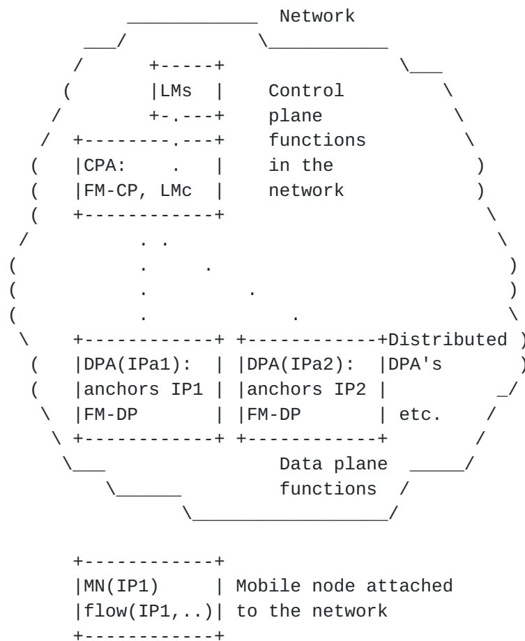
Figure 1. Configurations of network-based mobility management for a flat network to which MN is attached. The mobility management functions in the network are LMs in the control plane, LMc at CPA, and FM-DP at DPA.
