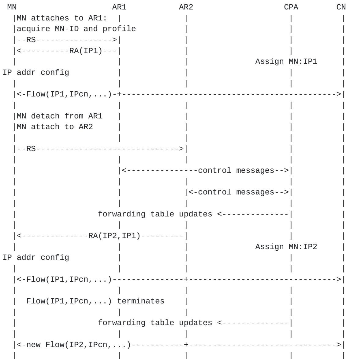
Figure 10. DMM solution. MN with flow using IP1 in Net1 continues to run the flow using IP1 as it moves to Net2.
