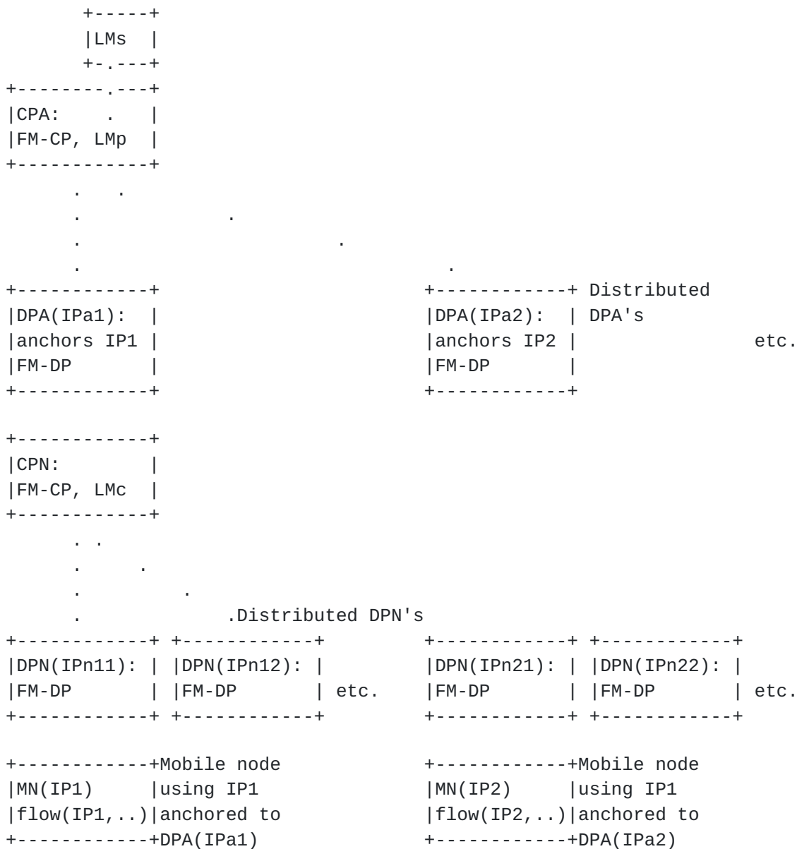
Figure 2. Configurations of network-based mobility management for a hierarchical network to which MN is attached. The mobility management functions in the network include a separate LMs, FM-CP and LMp at CPA, FM-DP at DPA; FM-CP and LMc at CPN, FM-DP at DPN.
