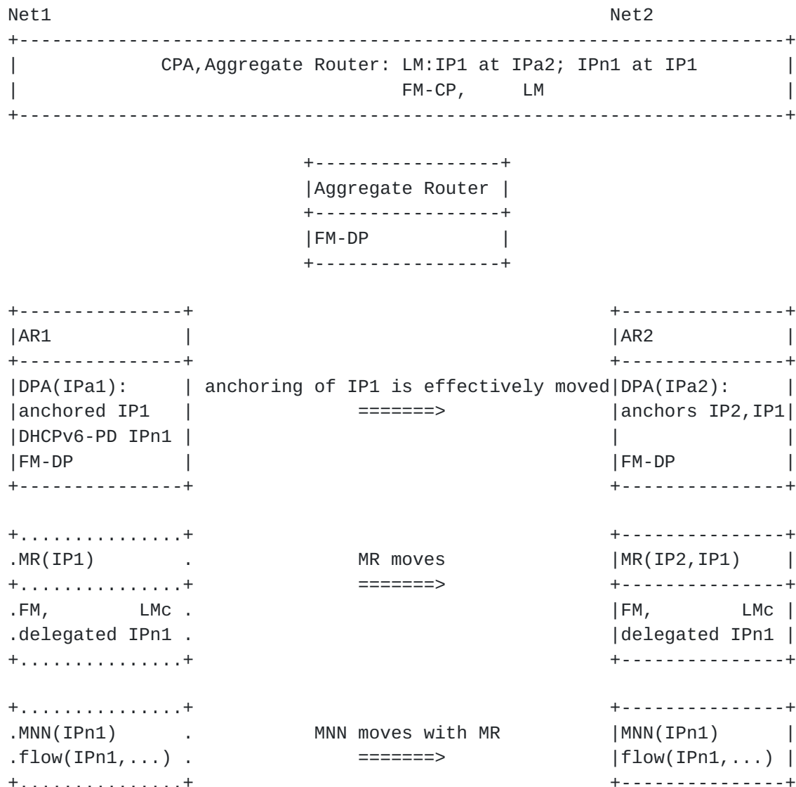
Figure 13. Mobility involving change of IP anchoring for a MR to which an MNN is attached.
