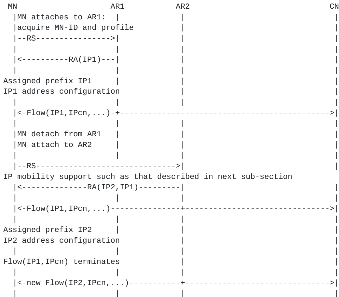
Figure 7. A flow continues to use the IP prefix from its home network after MN has moved to a new network.
