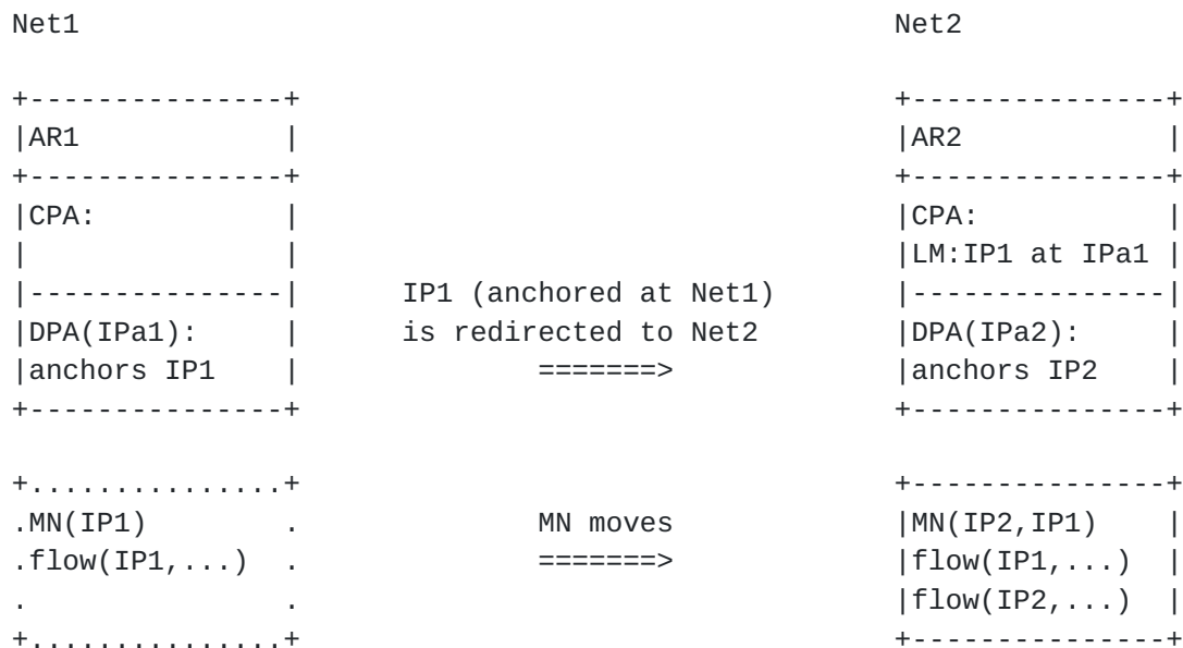
Figure 5: Anchor redirection
