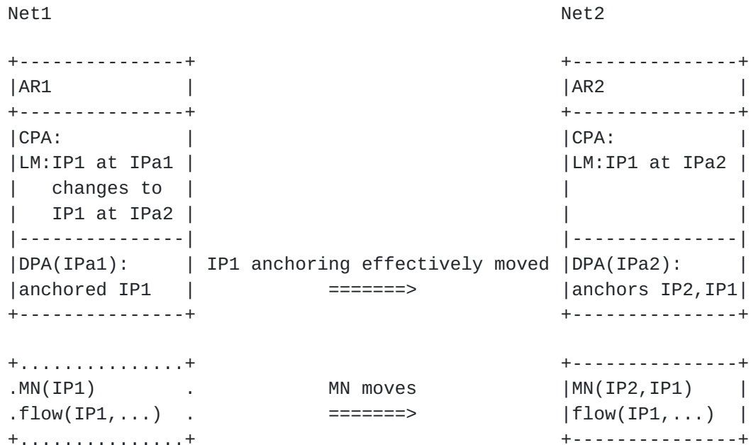
Figure 7: Anchor relocation
