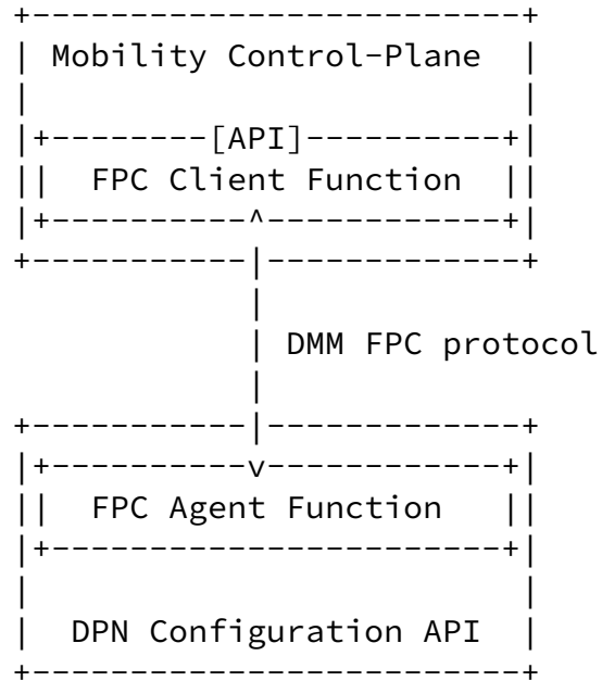
Figure 2: Functional reference architecture for DMM Forwarding Policy Configuration (FPC)
