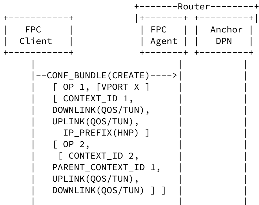
Figure 23: Exemplary Bundle Message (focus on FPC reference point)
