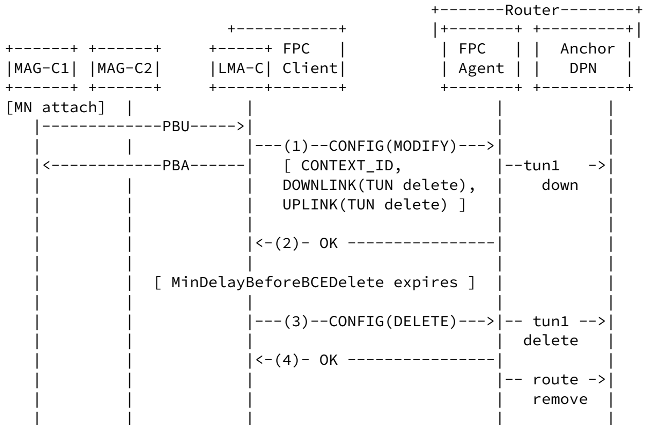
Figure 18: Exemplary Message Sequence (focus on FPC reference point)
