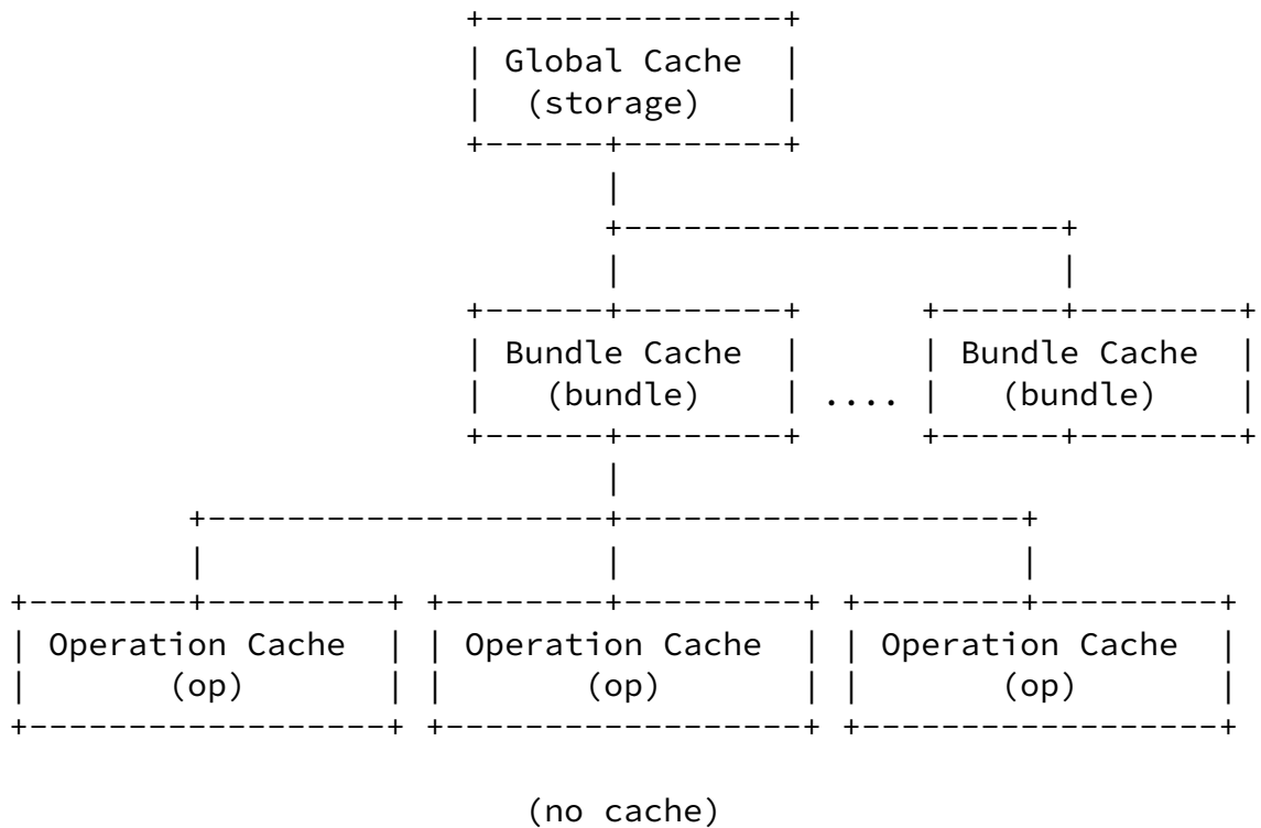
Figure 25: Exemplary Hierarchical Cache
