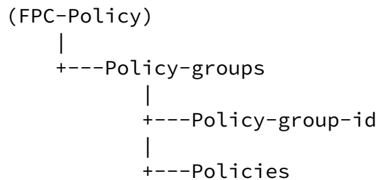
Figure 10: Policy-group Model Structure
