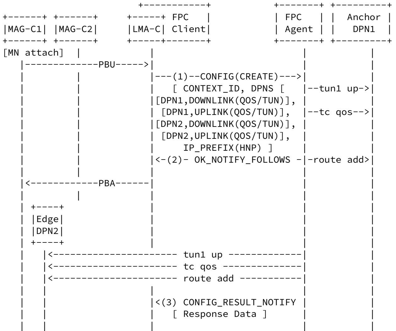
Figure 19: Exemplary Message Sequence for Multi-DPN Agent
