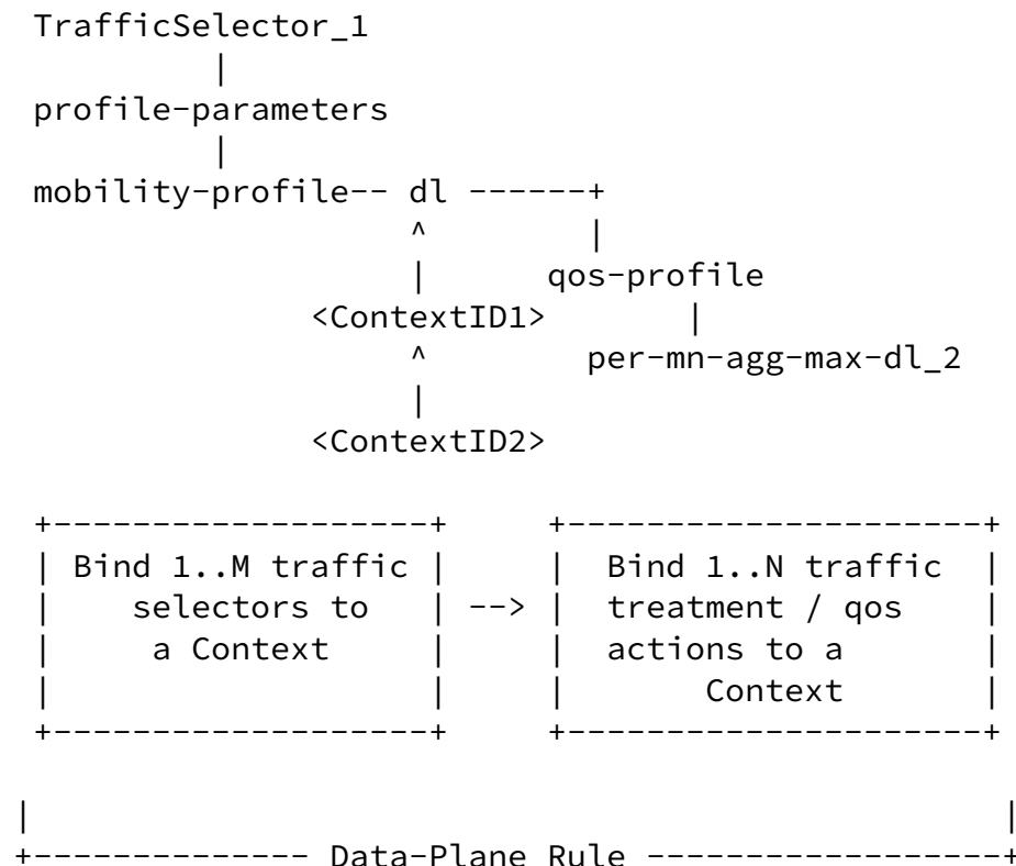
Figure 21: Structure of Contexts
