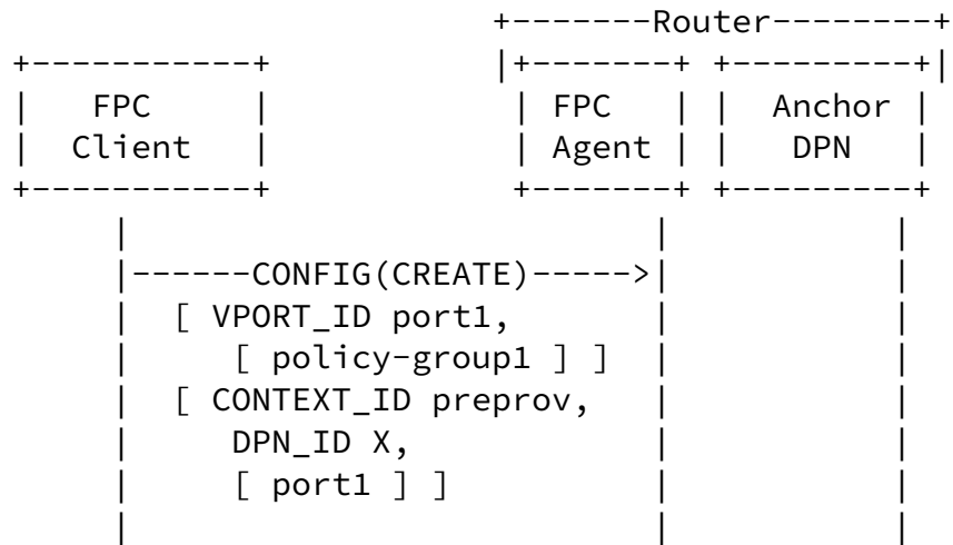
Figure 26: Exemplary Config Message for policy pre-provisioning
