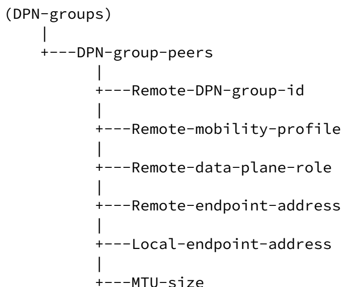
Figure 5: DPN-groups Peer Model Structure
