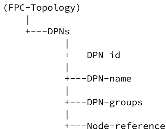
Figure 3: DPNs Model Structure
