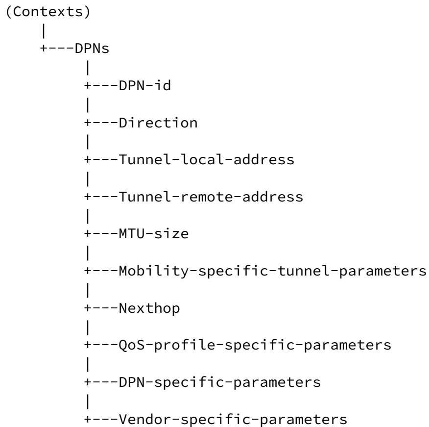
Figure 15: Multiple-DPN Supported Context Model Structure
