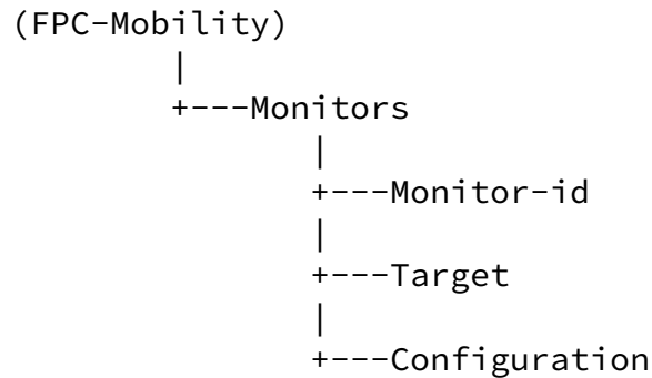
Figure 16: Common Monitor Model Structure
