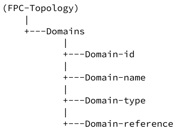
Figure 6: Domain Model Structure
