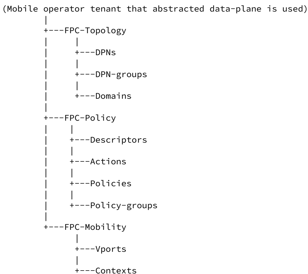
Figure 2: FPC Data-plane Information Model
