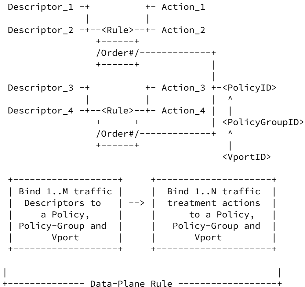
Figure 20: Structure of Policies and Vports
