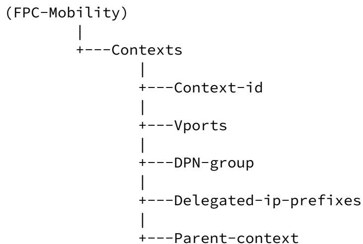
Figure 12: Common Context Model Structure
