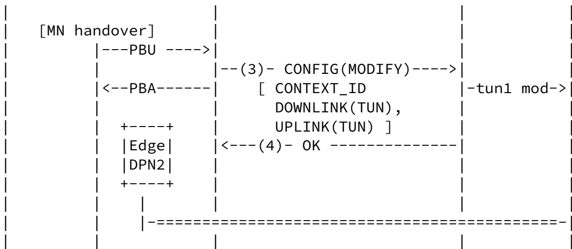
Figure 17: Exemplary Message Sequence (focus on FPC reference point)
