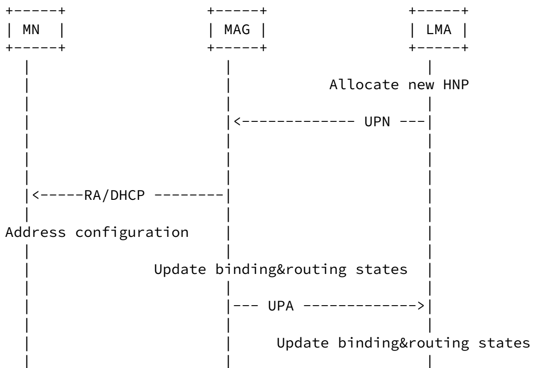
Figure 1: Signaling call flow of the HNP renumbering
