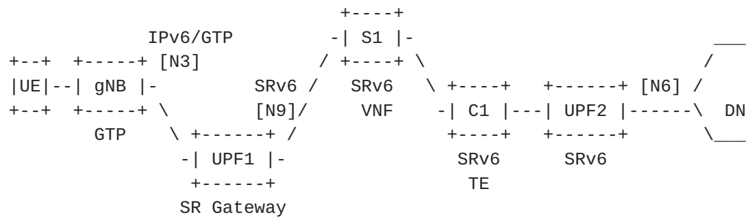
Figure 5: Enhanced mode with unchanged gNB IPv6/GTP behavior
