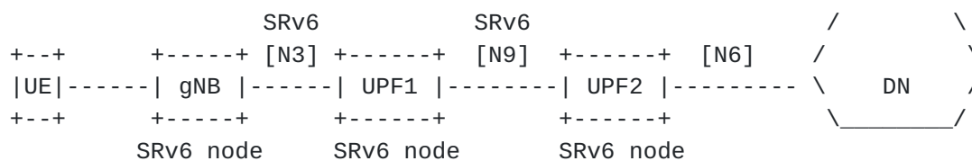
Figure 2: Traditional mode - example topology
