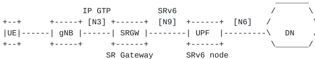
Figure 4: Example topology for interworking
