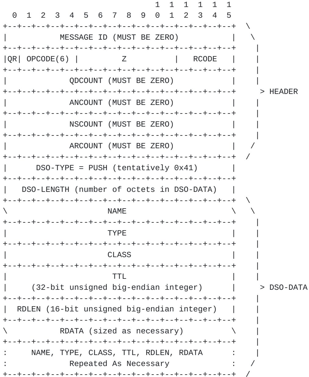
Figure 3: PUSH Message
