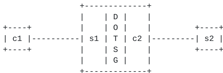
Figure 3: DOTS gateway
