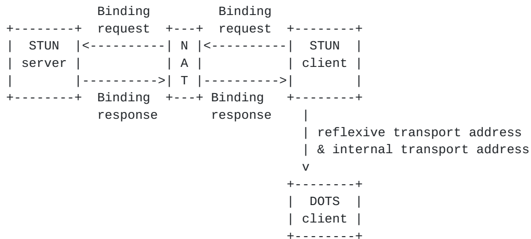
Figure 13: Resolving mitigation scope with STUN
