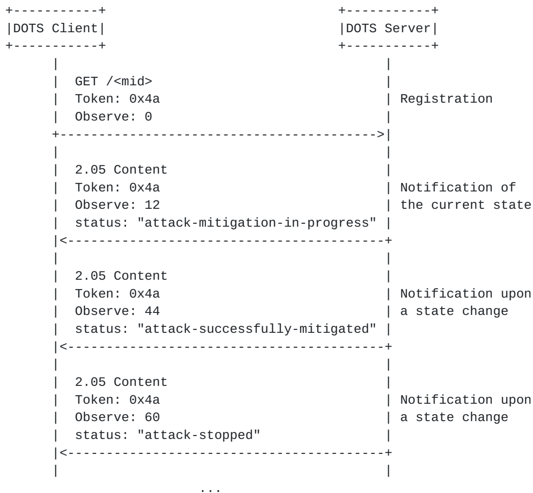
Figure 15: Notifications of Attack Mitigation Status
