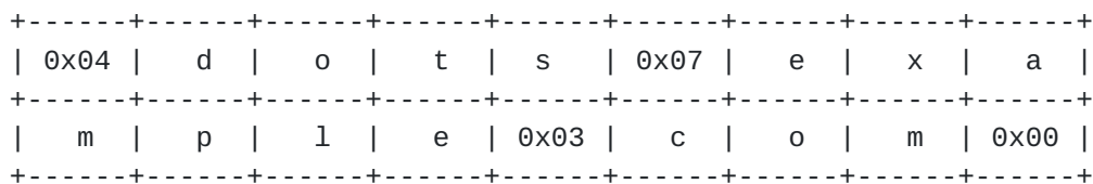
Figure 4: An example of the dots-agent-name Encoding
