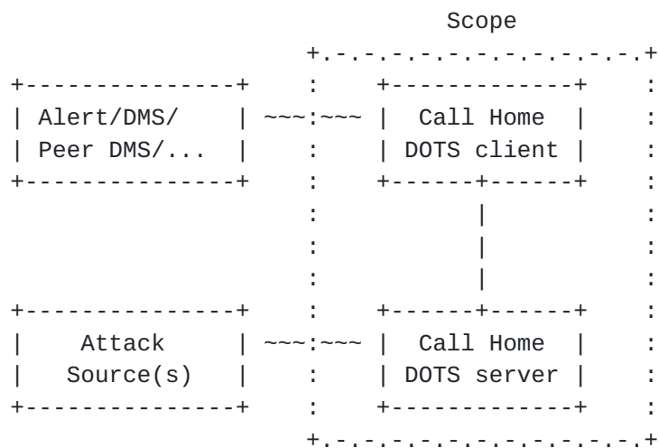
Figure 1: Basic DOTS Signal Channel Call Home Functional Architecture
