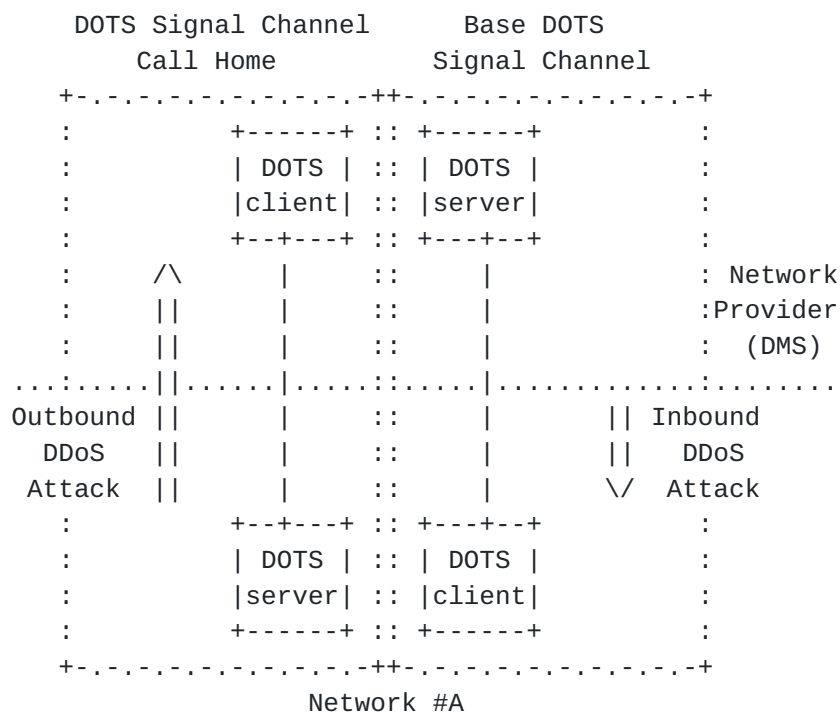
Figure 3: Activation of Base DOTS Signal Channel and Call Home (Same DMS Provider)
