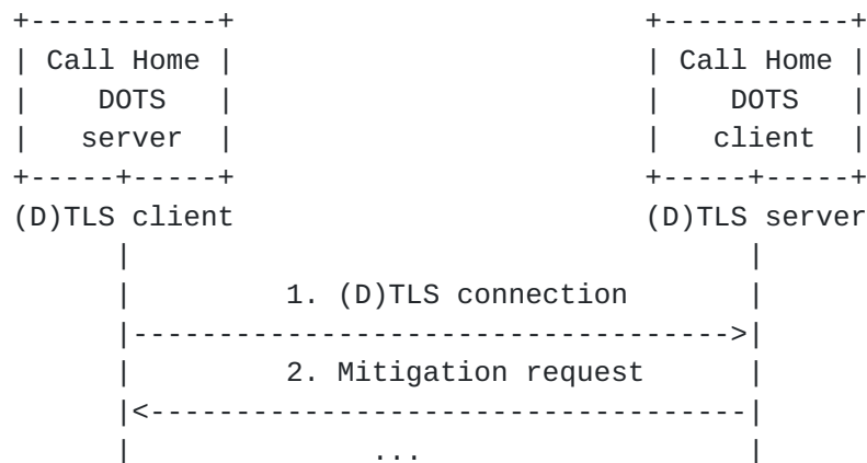
Figure 7: DOTS Signal Channel Call Home Sequence Diagram
