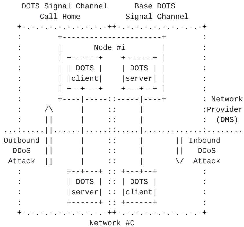
Figure 5: An Example of the Same Node Embedding both a Call Home DOTS Client and a DOTS Server at the Network Provider's Side
