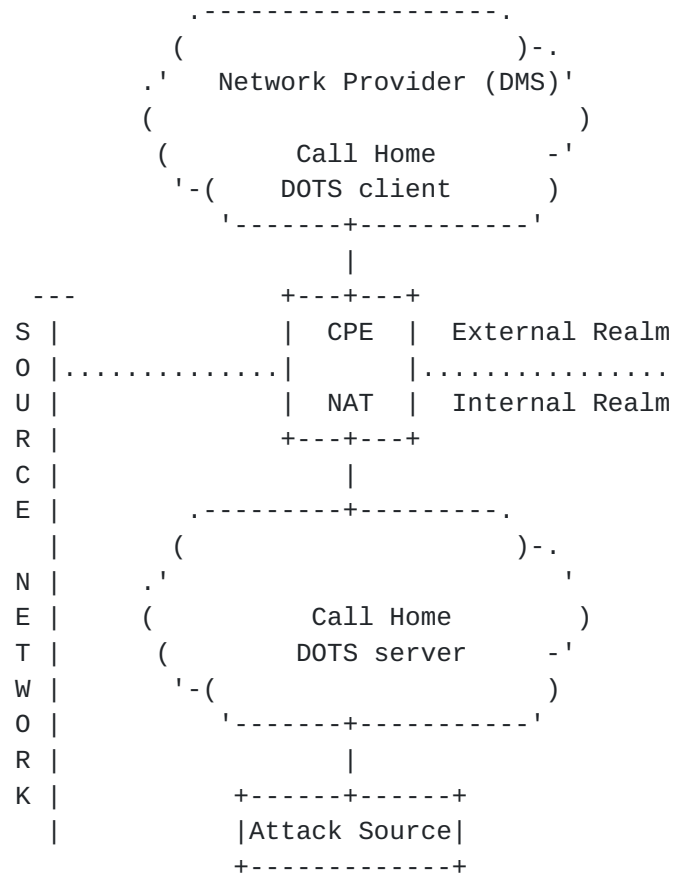
Figure 11: Example of a DOTS Server Domain with a NAT Embedded in a CPE
