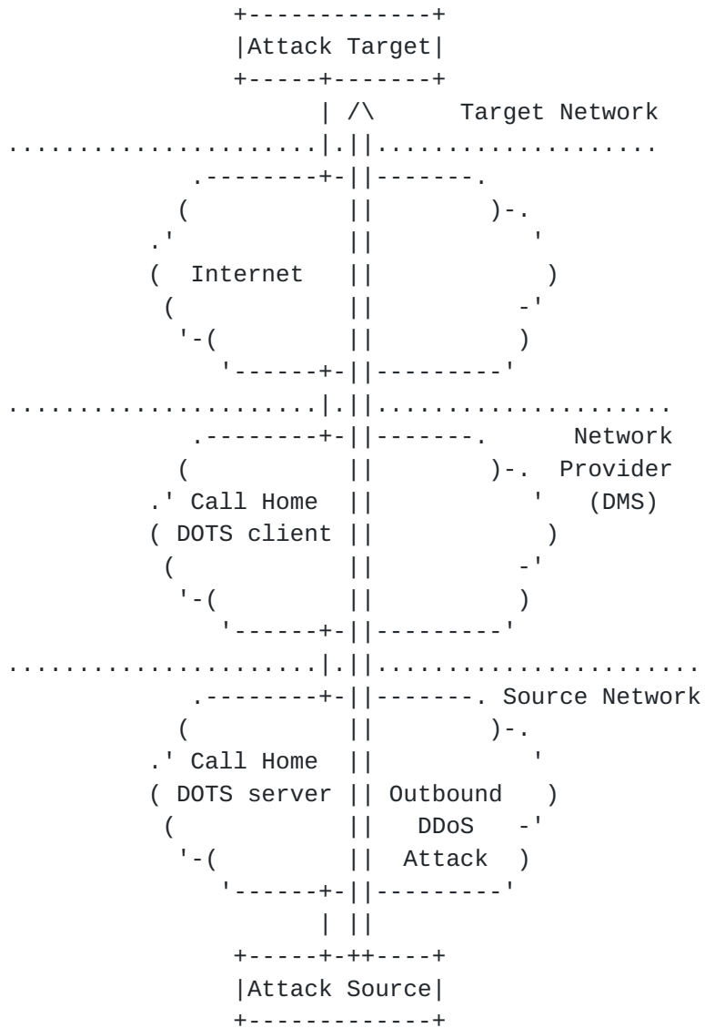
Figure 2: DOTS Signal Channel Call Home Reference Architecture
