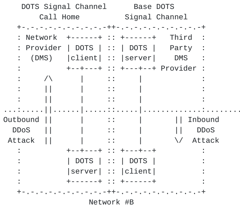
Figure 4: Activation of Base DOTS Signal Channel and Call Home (Distinct DMS Providers)
