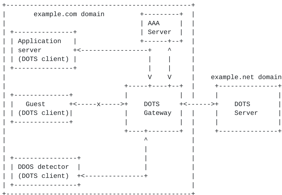
Figure 22: Example of Authentication and Authorization of DOTS Agents
