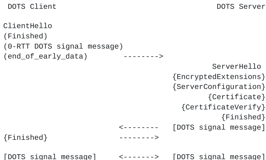
Figure 21: TLS 1.3 handshake with 0-RTT
