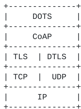
Figure 3: Abstract Layering of DOTS signal channel over CoAP over (D)TLS
