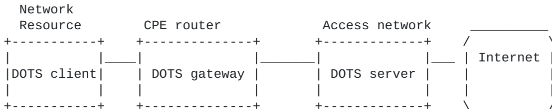
Figure 1: Sample DOTS Deployment (1)
