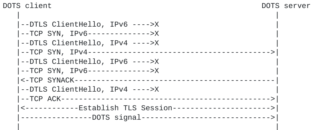
Figure 4: DOTS Happy Eyeballs
