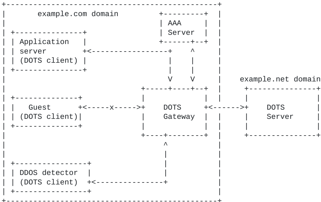
Figure 24: Example of Authentication and Authorization of DOTS Agents
