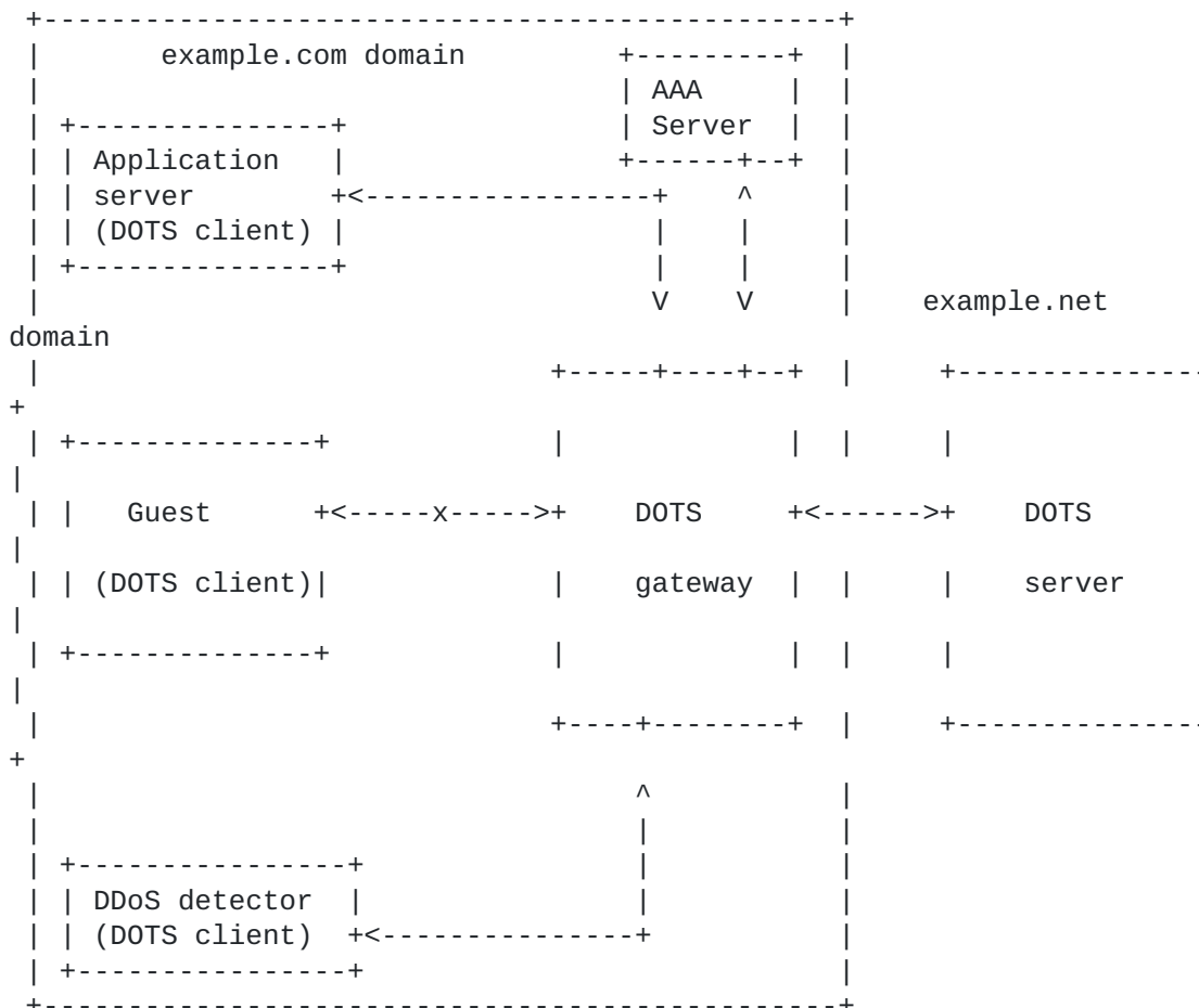
Figure 25: Example of Authentication and Authorization of DOTS Agents
