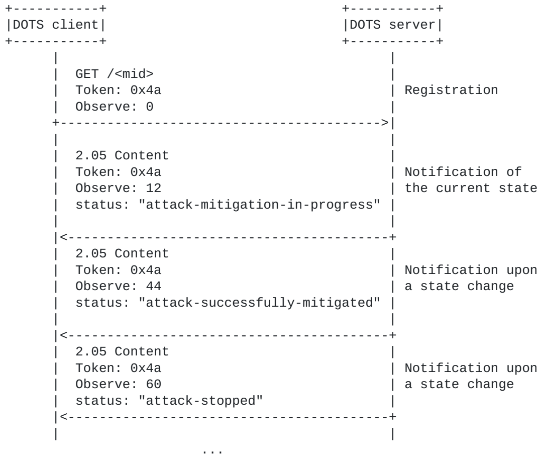
Figure 15: Notifications of Attack Mitigation Status
