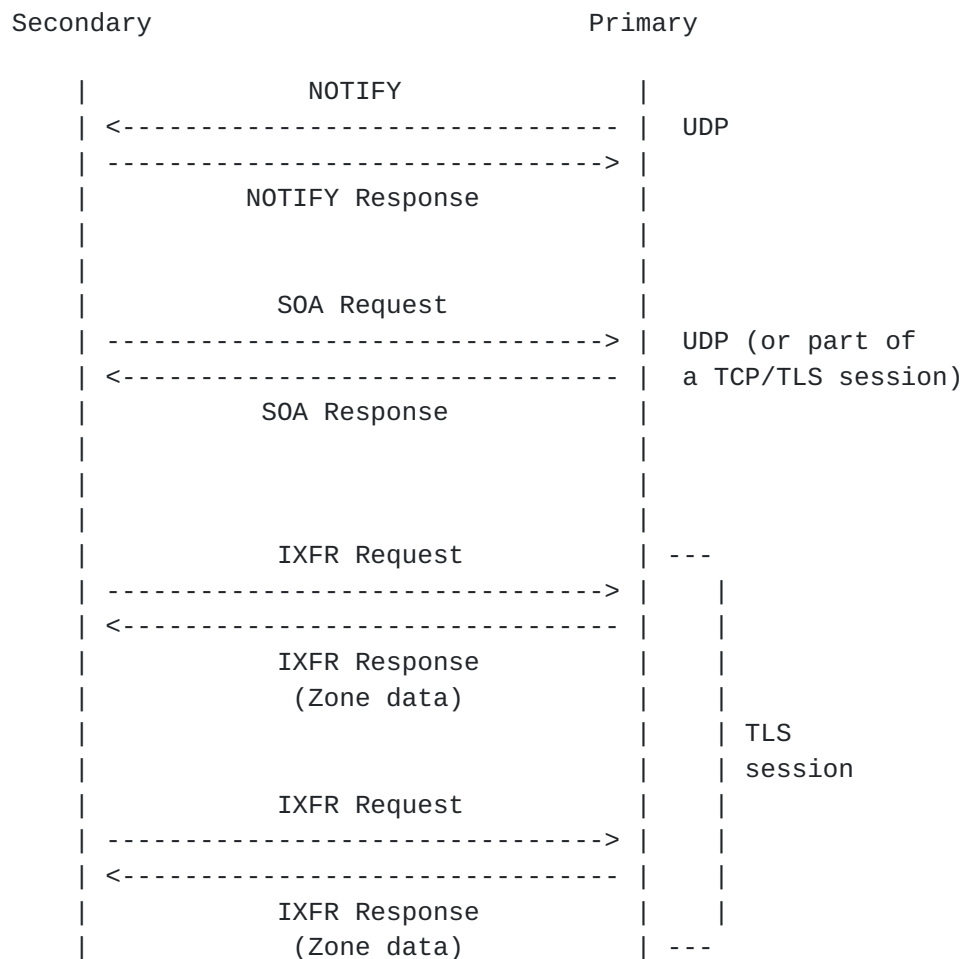
Figure 1. IXoT Mechanism
