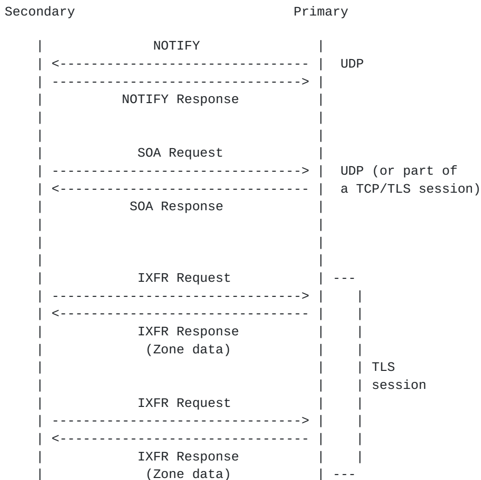
Figure 4. IXoT Mechanism
