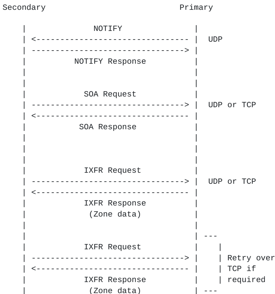
Figure 2. IXFR Mechanism
