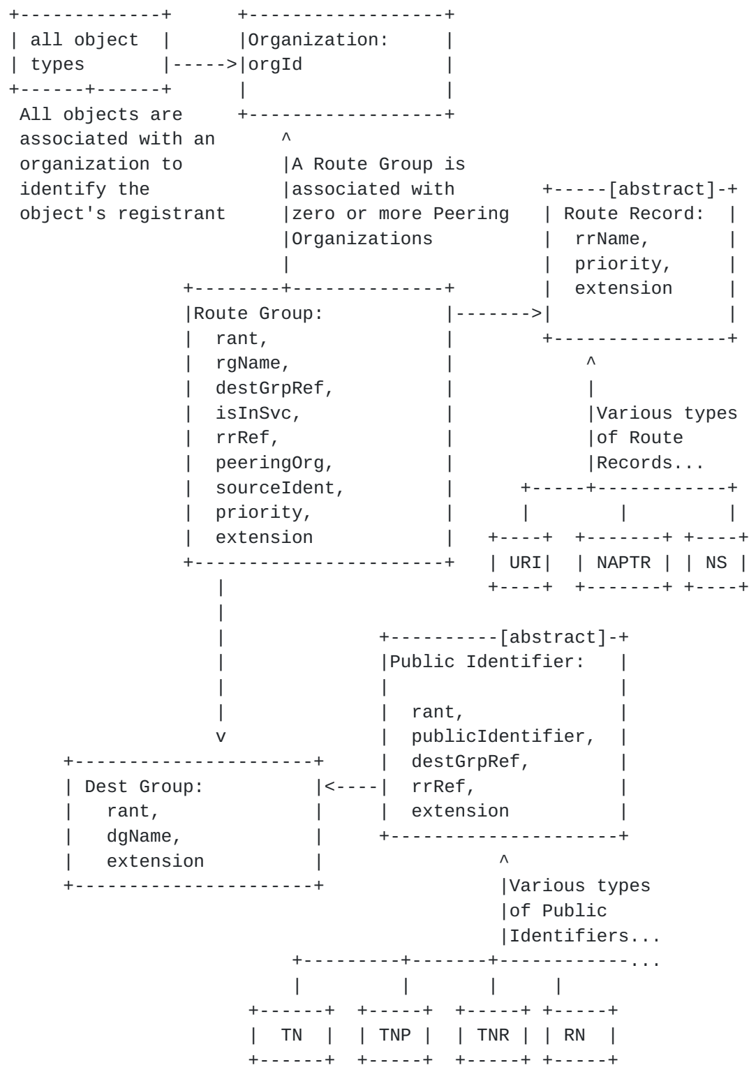
SPPF Data Model
