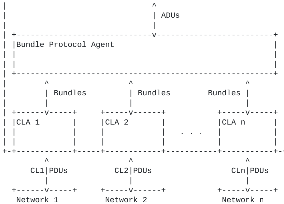
Figure 2: Components of a Bundle Node
