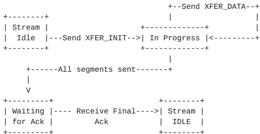
Figure 11: Transfer sender states
