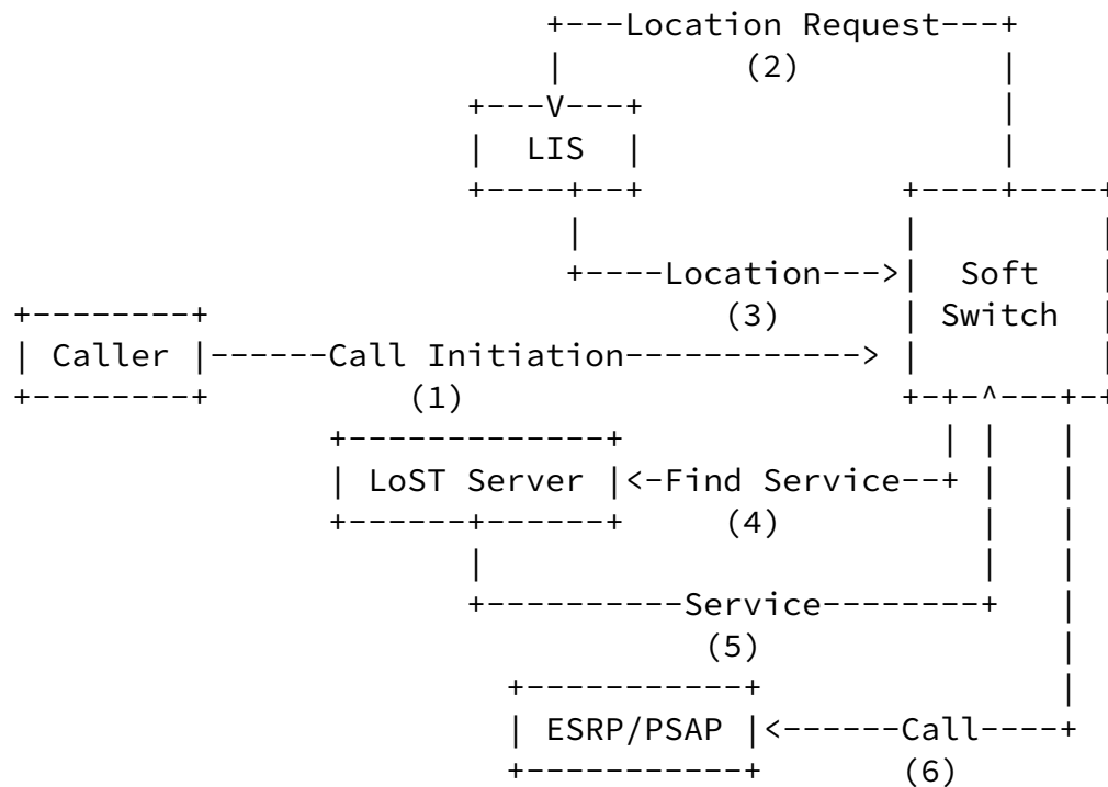
Figure 2: Softswitch-Centric Calling Model
